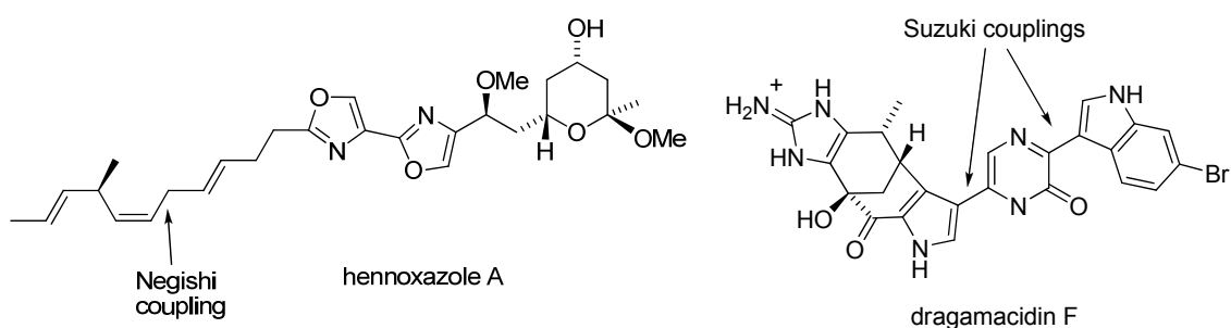
Figure 1. Synthesis of hennoxazole A (ref 34) and dragmacidin F (ref 35) via palladium-catalyzed cross coupling.
