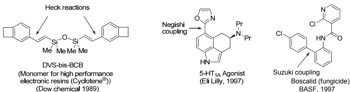
Figure 2. Palladium-catalyzed cross-coupling reactions in industrial preparation of fine chemicals: DVS-bis-BCB (Cyclotene®) (ref. 37), 5-HT 1A Agonist (ref. 38), and Boscalid (ref 39)
