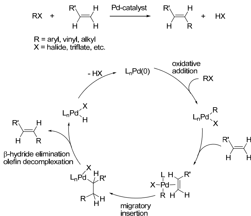
Scheme 1. Mechanism of the Heck reaction.
