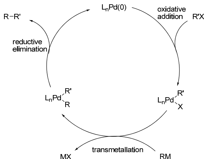
Scheme 2. Mechanism of the Negishi and Suzuki palladium-catalyzed cross-coupling reactions.
