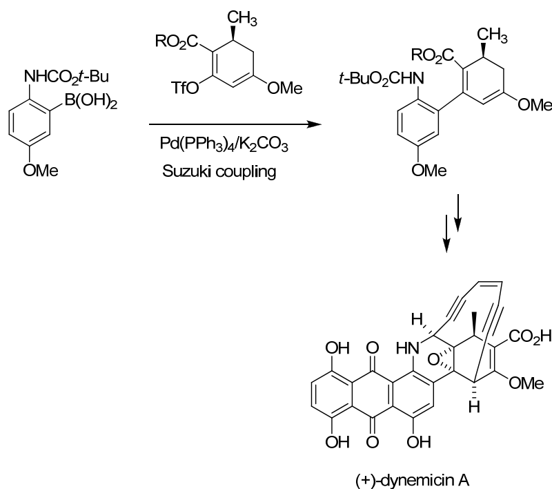
Scheme 5. An efficient Suzuki coupling in the synthesis of (+)-dynemicin A (ref. 33).
