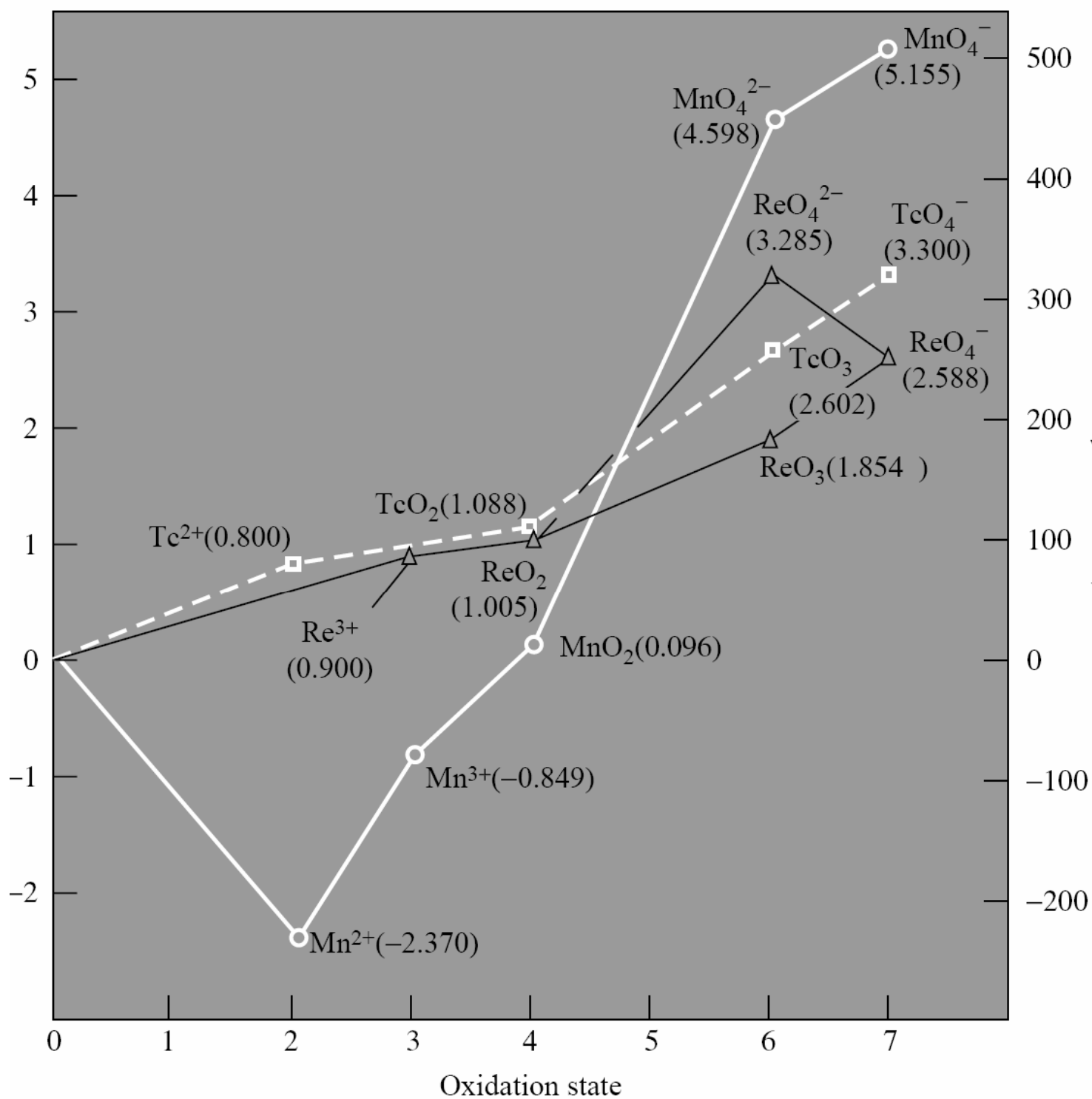
Figure 24.1 Plot of volt-equivalent versus oxidation state for Mn, Tc and Re.
