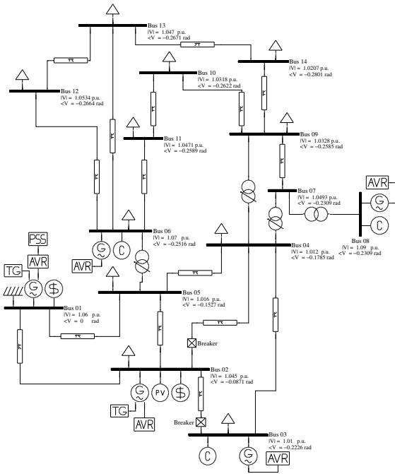
Fig. 7. PSAT-Simulink model of the IEEE 14-bus test system.
