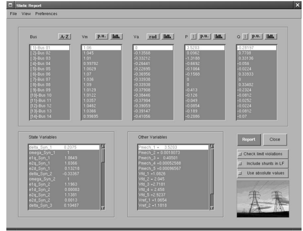
Fig. 6. GUI for power flow reports. The results refer to the IEEE 14-bus test system.
