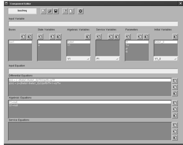
Fig. 5. GUI for user defined models.
