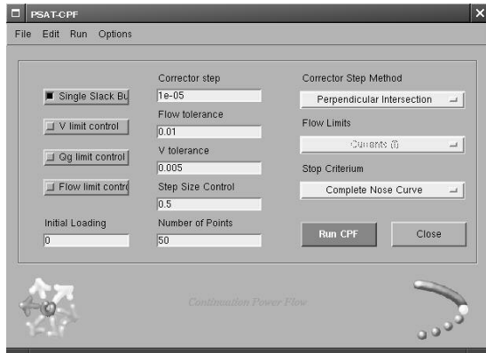
Fig. 8. GUI for continuation power flow settings.
