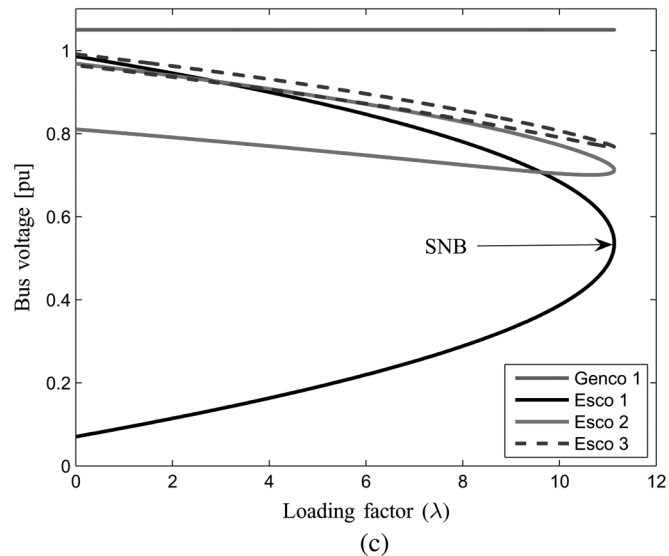
Fig. 3. Generators' PV curves for the six-bus test system. (a) Base case (LIBS preceded by LIDBs). (b) Line 2-4 outage (SNB preceded by LIDBs). (c) Base system neglecting reactive power limits (SNB).
